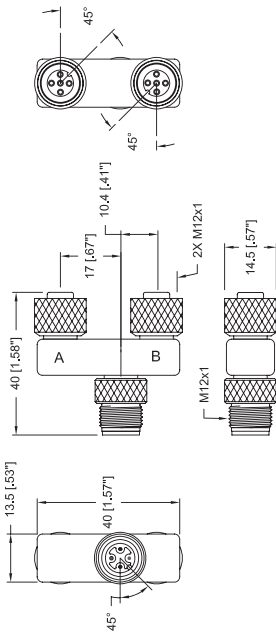
ASBS 2 M12-S2326
