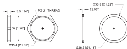
Panel Nut / Sealing Ring
