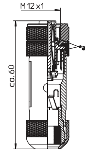
*a O-Ring
